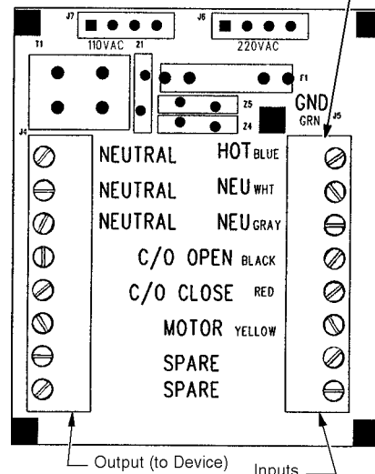
Lower PC Board: AC Input
